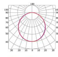
Opal cover with fins (light reduction: -26%)
