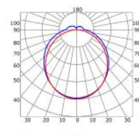
Frosted cover (light reduction: -24%)
