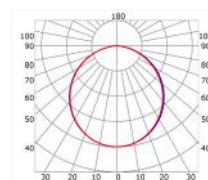
Opal cover: -53% Frosted cover: -59%
