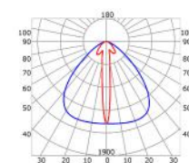
11° lens cover (light reduction -37%)
