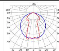
Transparent cover (light reduction -35%)
