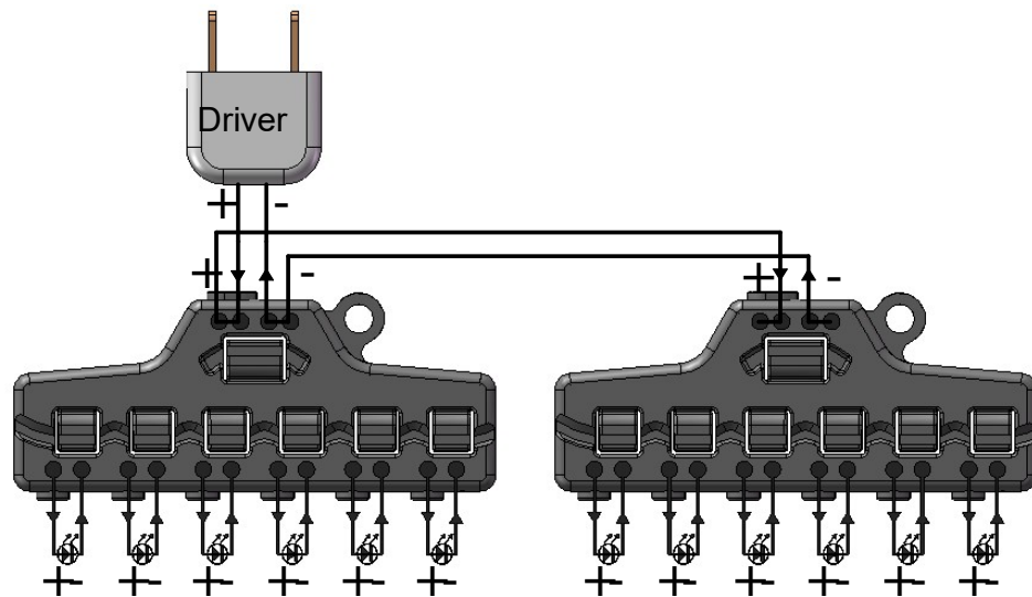
CP-FC6-2 Constant Voltage Connection
